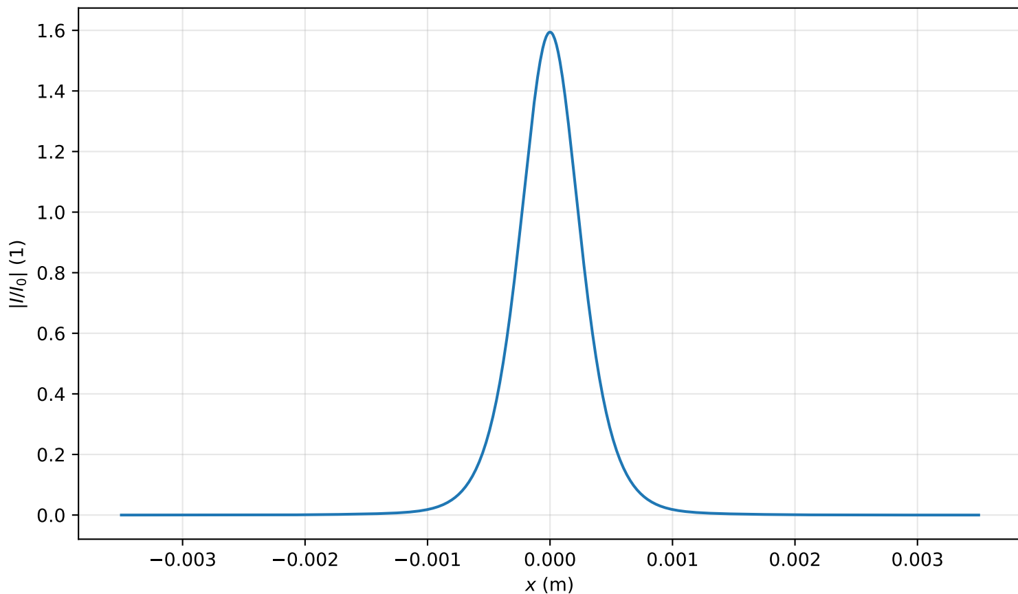
Intensity profile I(x, y = 0, z = 2.786m)/I_0 , P_{in}=0.9P_{cr} , artificial time
